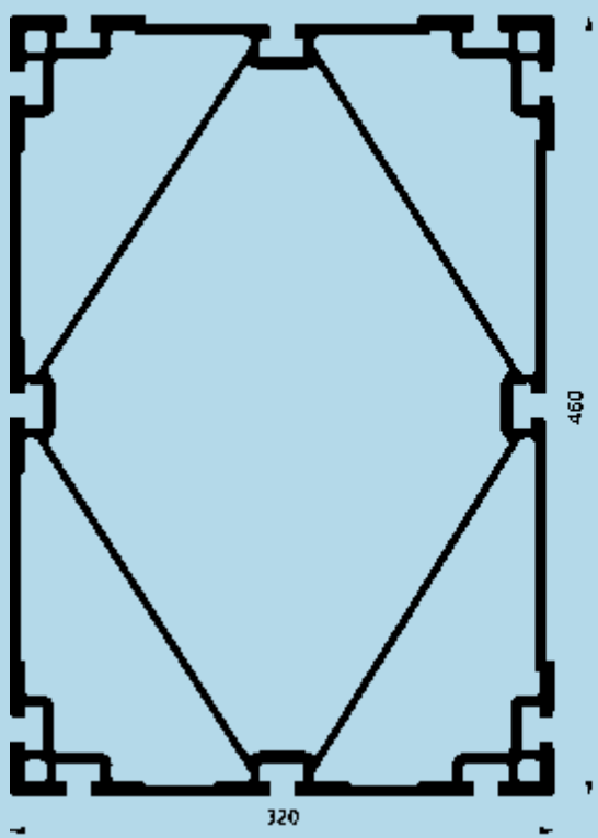
NTS 46x32 I die No. 41747 G=51,05 kg/m
